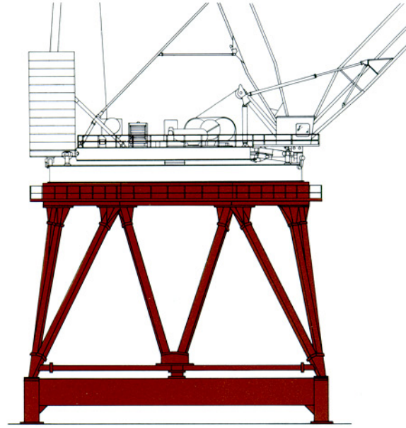
GANTRY MOUNT
