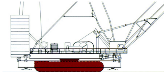
CRAWLER-TRANSPORTER
